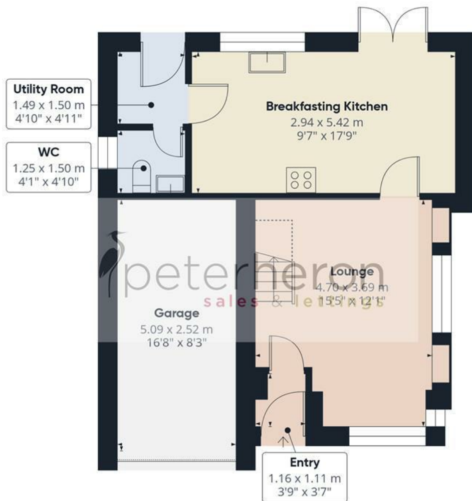
Ground Floor
